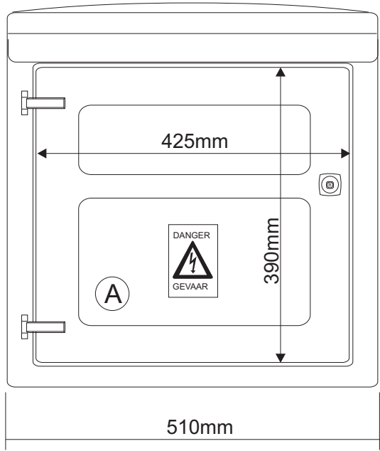
Wall Mount
