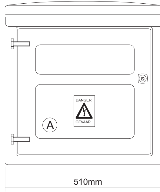
Pole Mount
