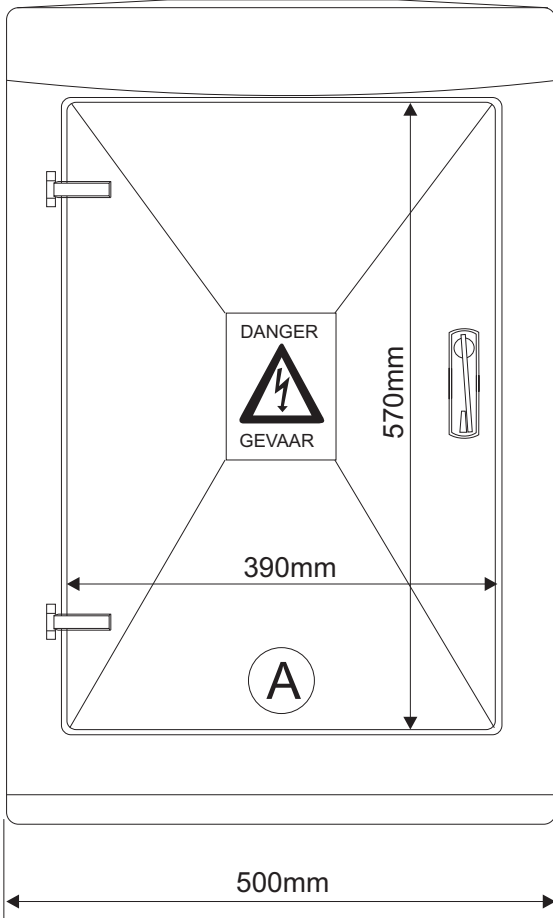
Wall Mount
