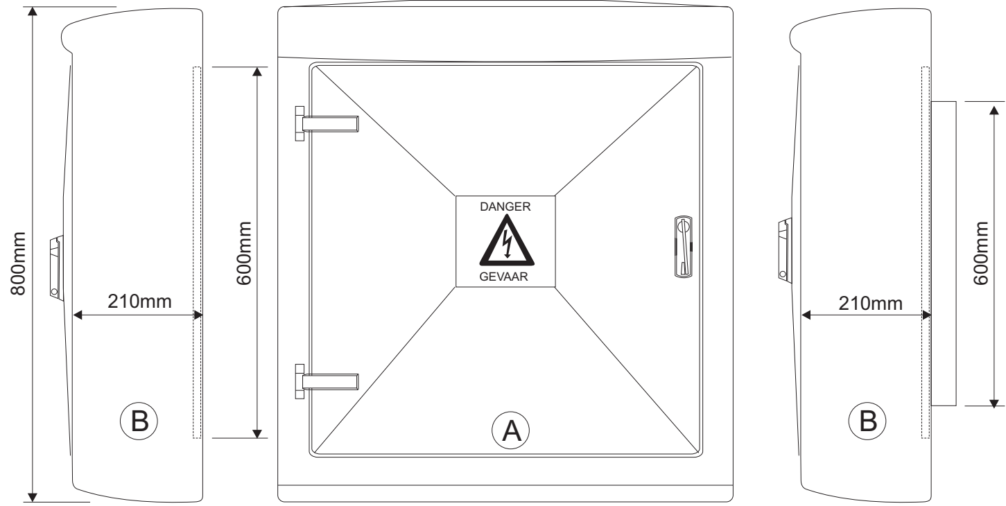
Pole Mount
