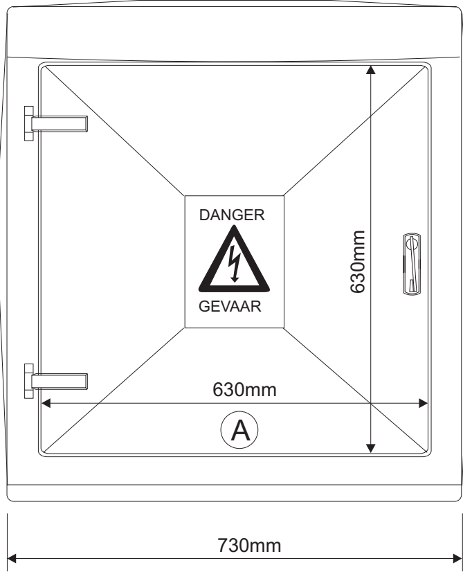
Wall Mount
