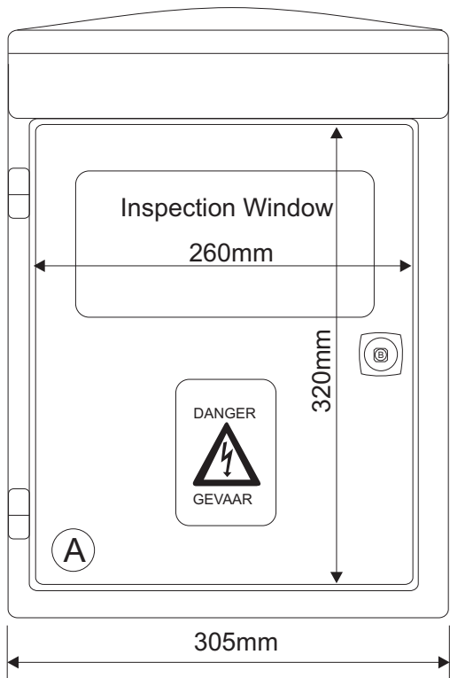
Wall Mount
